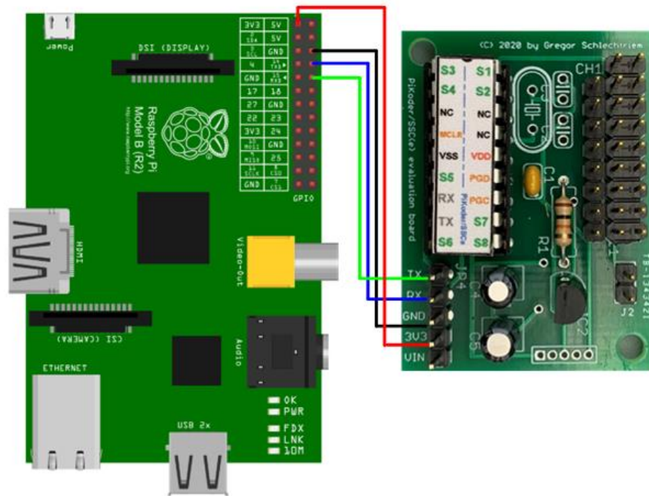
Wiring scheme for connecting your PiKoder/SSCe to a Raspberry Pi
